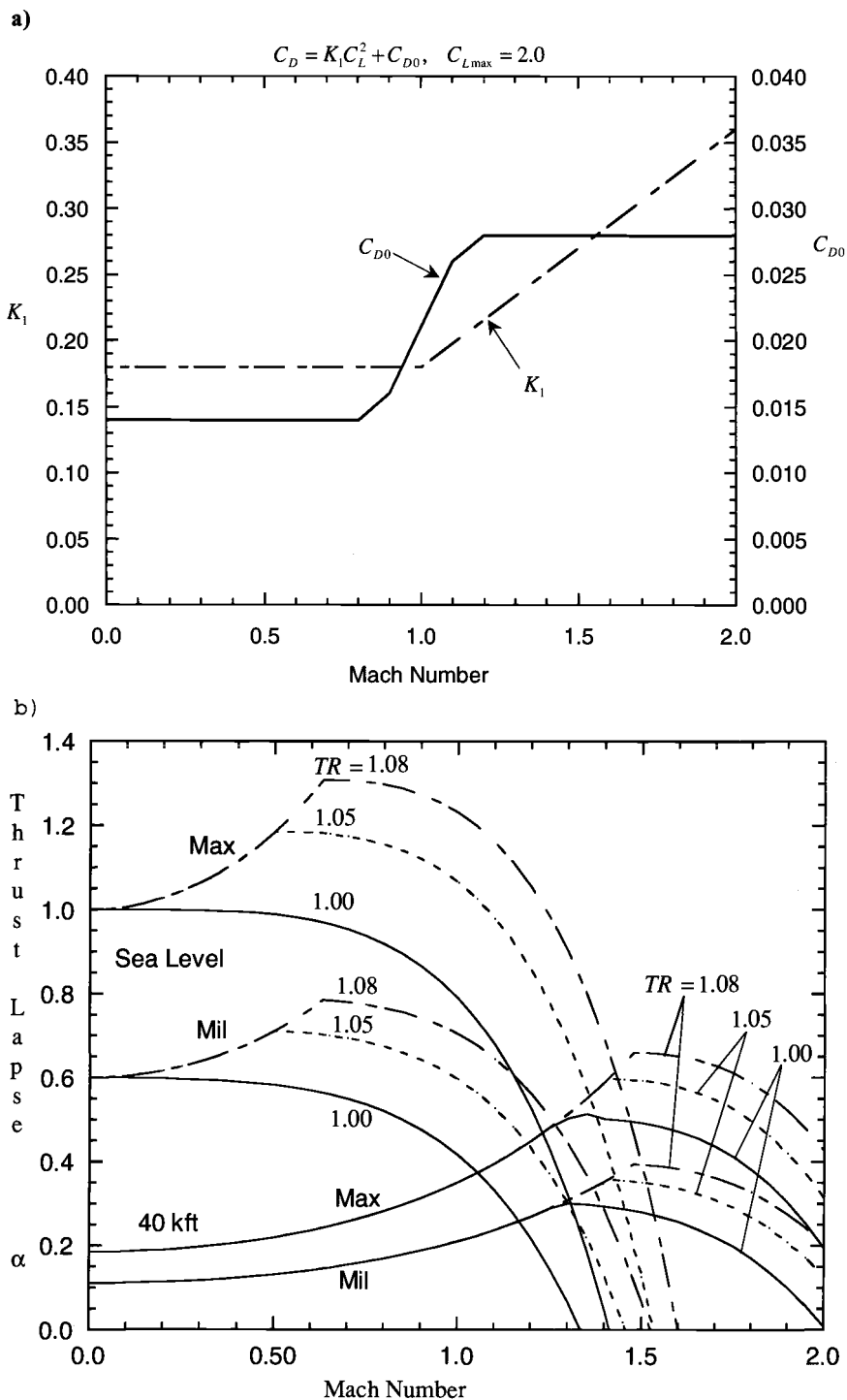
Fig. 2.E1 Preliminary AAF data: a) aerodynamic data; b) installed thrust lapse.
