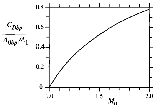
Fig. 10.27 Bypass drag of model pitot inlet (Fig. 10.24) with M_e = 1 and \phi = 0 deg.
