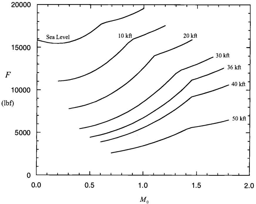
Fig. 6.E8 AAF Engine thrust at maximum power (standard day).
