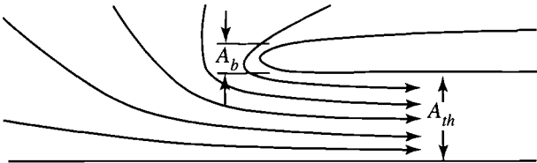
Fig. 10.19 Rounded lip inlet at zero flight speed.
