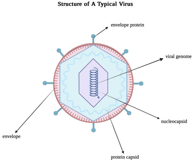
Figure 1. Structure of a virus. The figure above shows the typical structure that viruses have. While not all viruses have envelopes, they have a capsid and a viral genome made of RNA or DNA.
