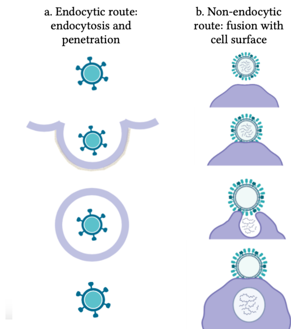
Figure 3. Endocytosis and fusion. The figure above shows the endocytic (left) and the non-endocytic (right) route, the two different ways animal viruses with envelopes can enter a cell. Adapted from (Dimitrov, 2004).
