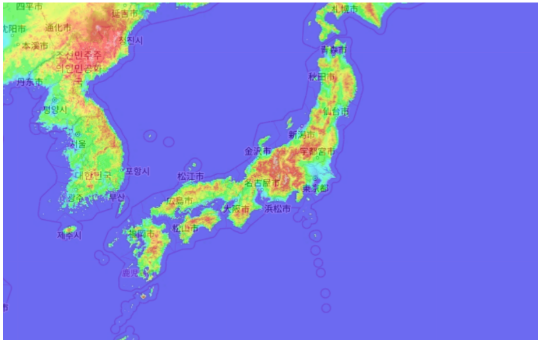
Figure 3: Elevation Heat Map of Japan ( https://en-gb.topographic-map.com/ )
