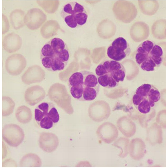
Figure 4: HTLV - 1 Positive Sample
